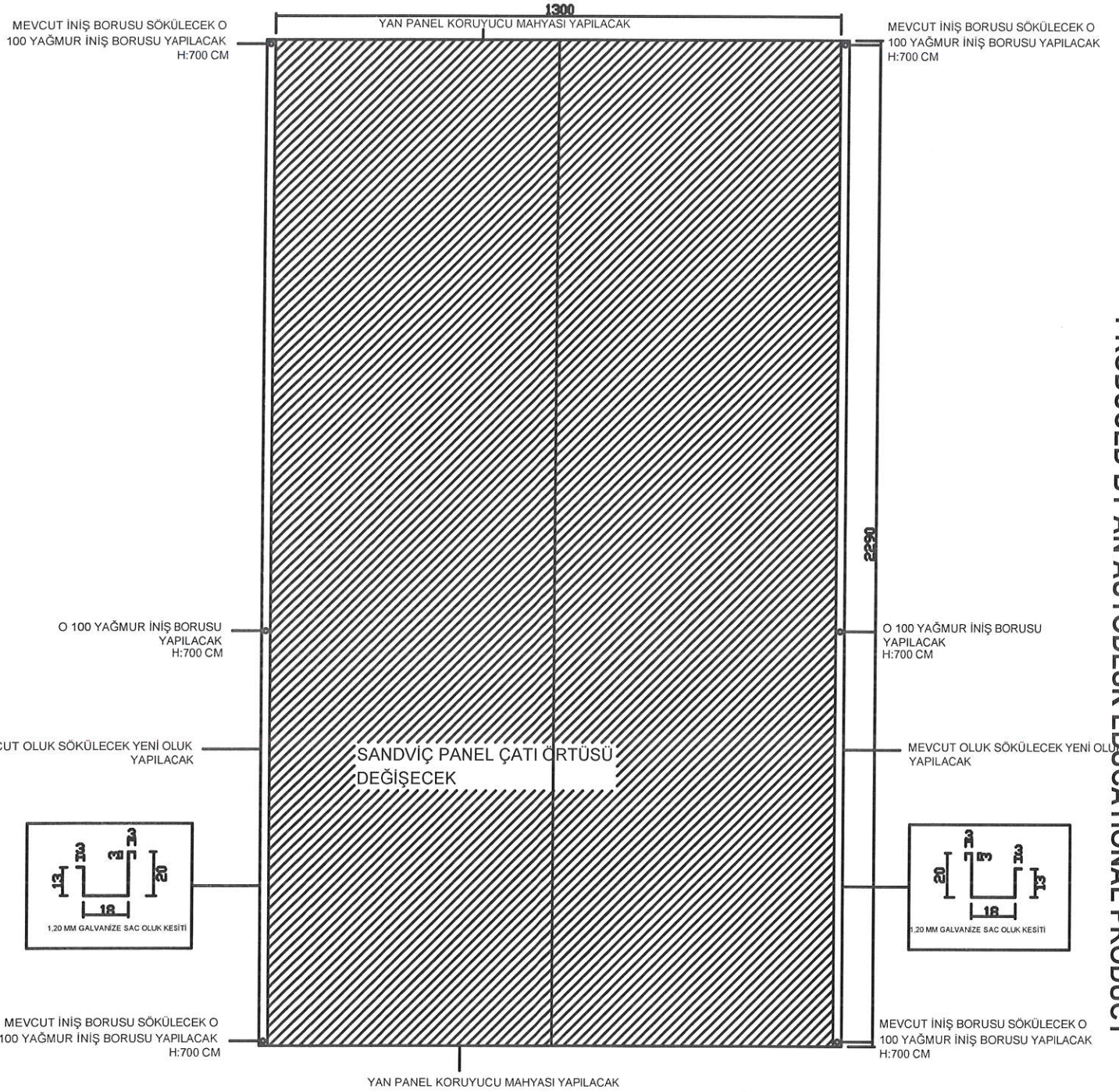
ÇATI PLANI
