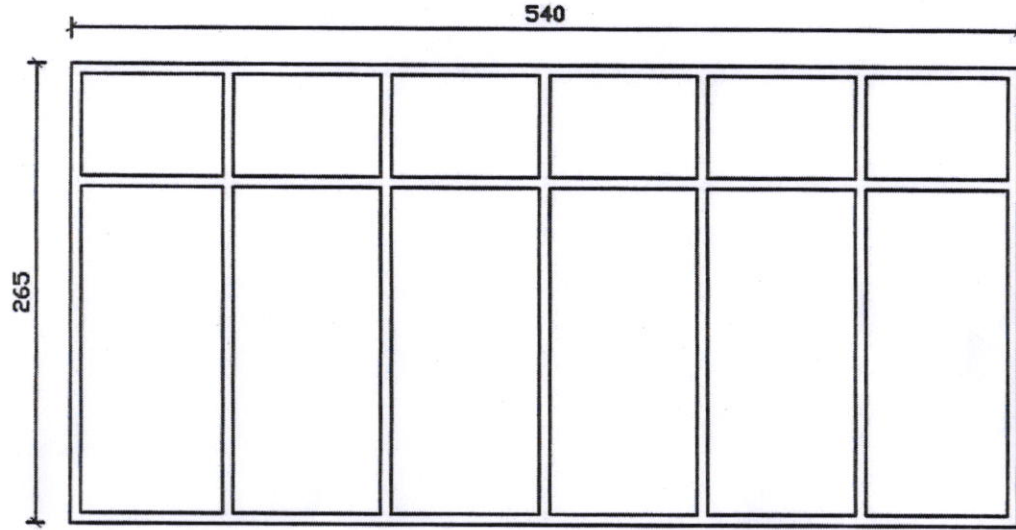
540/265 ALUMINYUM DOGRAMA
