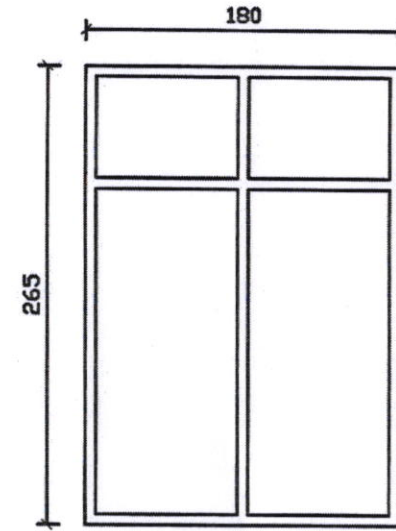
180/265 ALUMINYUM DOGRAMA
